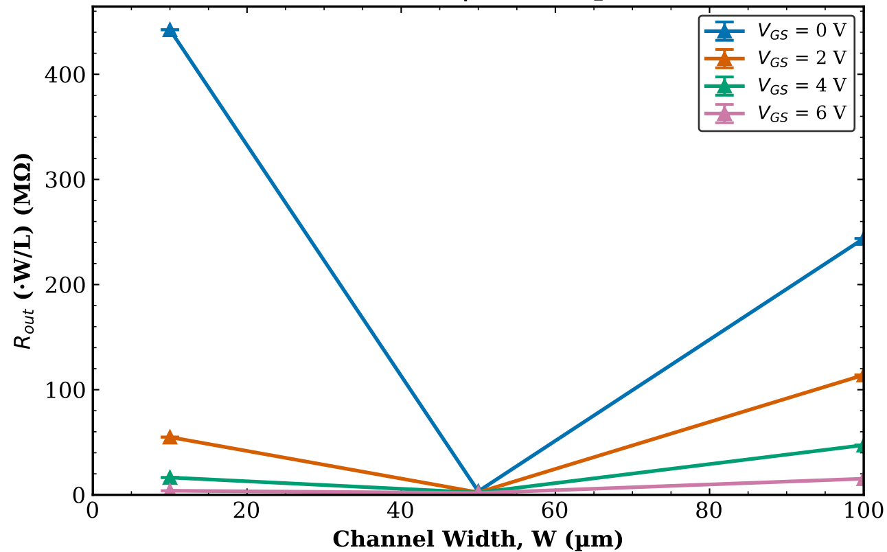
TFT3 Transistor 2 R_{out} vs W | L = 20\text{ }\mu\text{m}
